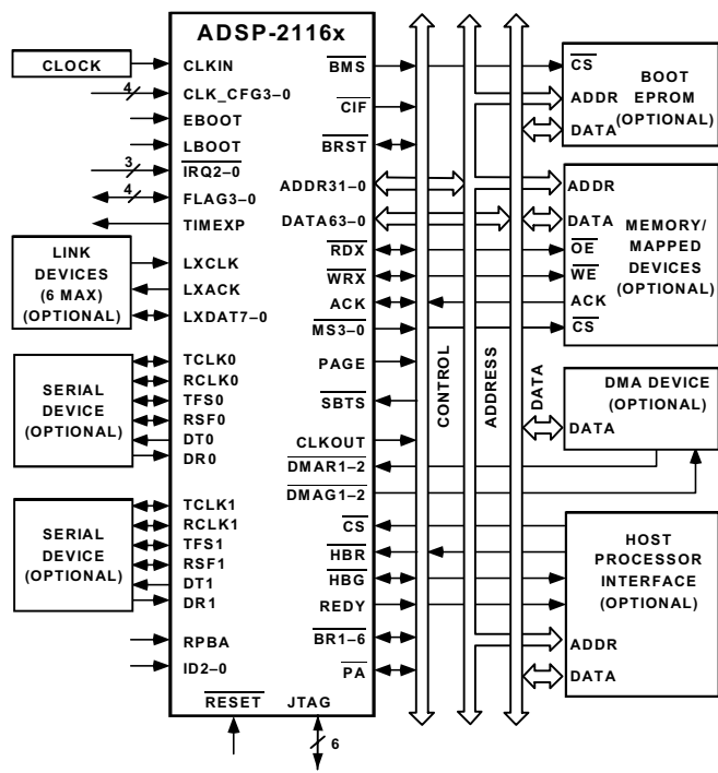
Figure 1. Single-Processor System
