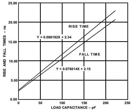
Figure 34. Typical Output Rise Time (10%-90%, V_{DDEXT} = Min ) vs. Load Capacitance
