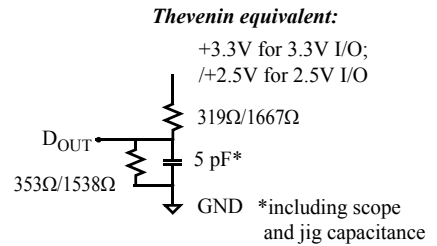
Figure C: Output load(B)
