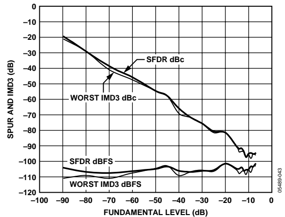
Figure 41. AD9445-105 Two-Tone SFDR vs. Analog Input Level 105 MSPS/30.3 MHz, 31.3 MHz
