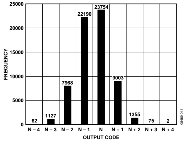
Figure 42. AD9445-125 Grounded Input Histogram
