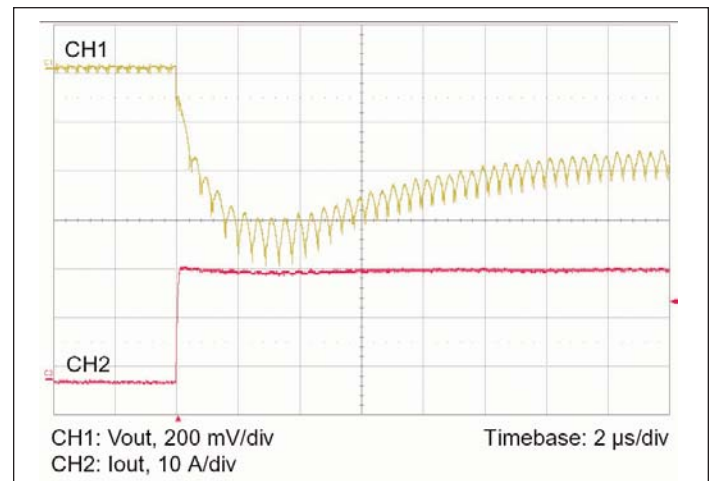
Figure 10 — 0-25 A load step with 47 μF input capacitor and no output capacitor.
