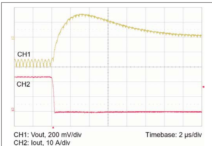
Figure 11 — 25-0 A load step with 47 μF input capacitance.
