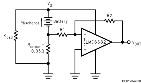
FIGURE 27. Circuit Used to Sense Discharging
