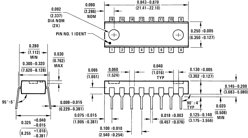
16-Pin Molded Dual-In-Line Package Order Number LMC6684AIN or LMC6684BIN NS Package Number N16A
