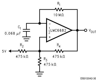
FIGURE 22. 1 Hz Square—Wave Oscillator
