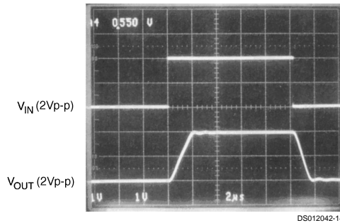
FIGURE 10. Pulse Response of the LMC6682 Circuit Shown in Figure 9
