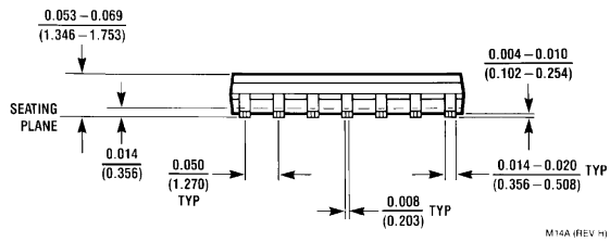
14-Pin Small Outline Package Order Number LMC6682AIM or LMC6682BIM NS Package Number M14A
