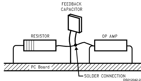
FIGURE 13. Air Wiring
