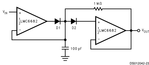
FIGURE 21. Low Voltage Peak Detector
