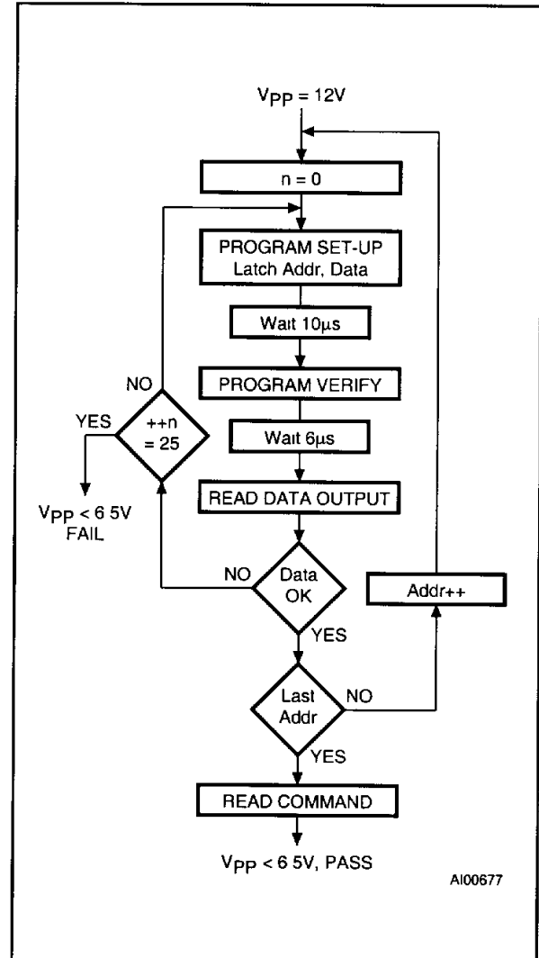
Figure 13. Programming Flowchart
