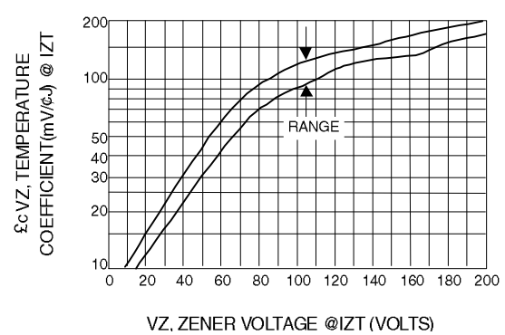
Fig. 6-UNITS 10 TO 200 VOLTS
