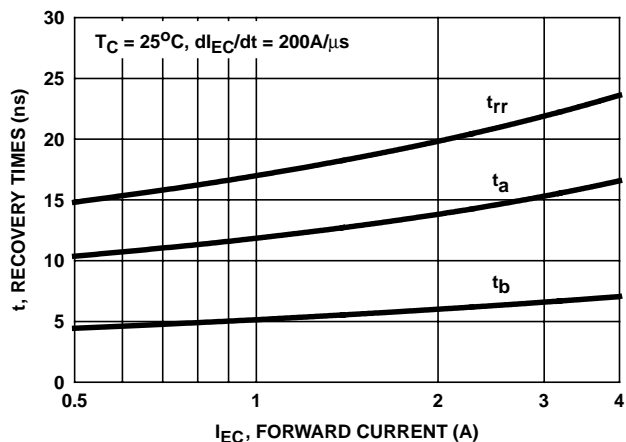
FIGURE 18. RECOVERY TIME vs FORWARD CURRENT
