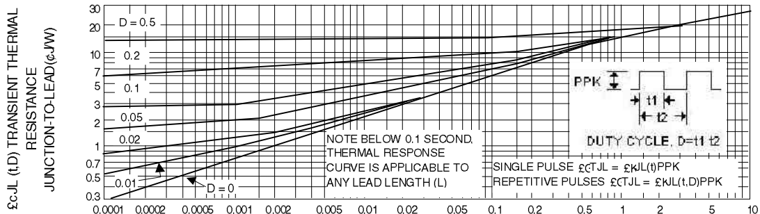
Fig. 2-TYPICAL THERMAL RESPONSE L,
