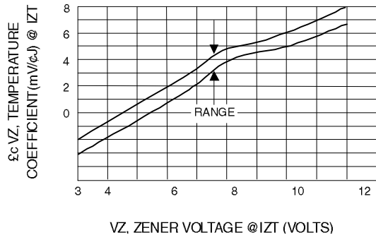
Fig. 5-UNITS TO 12 VOLTS
