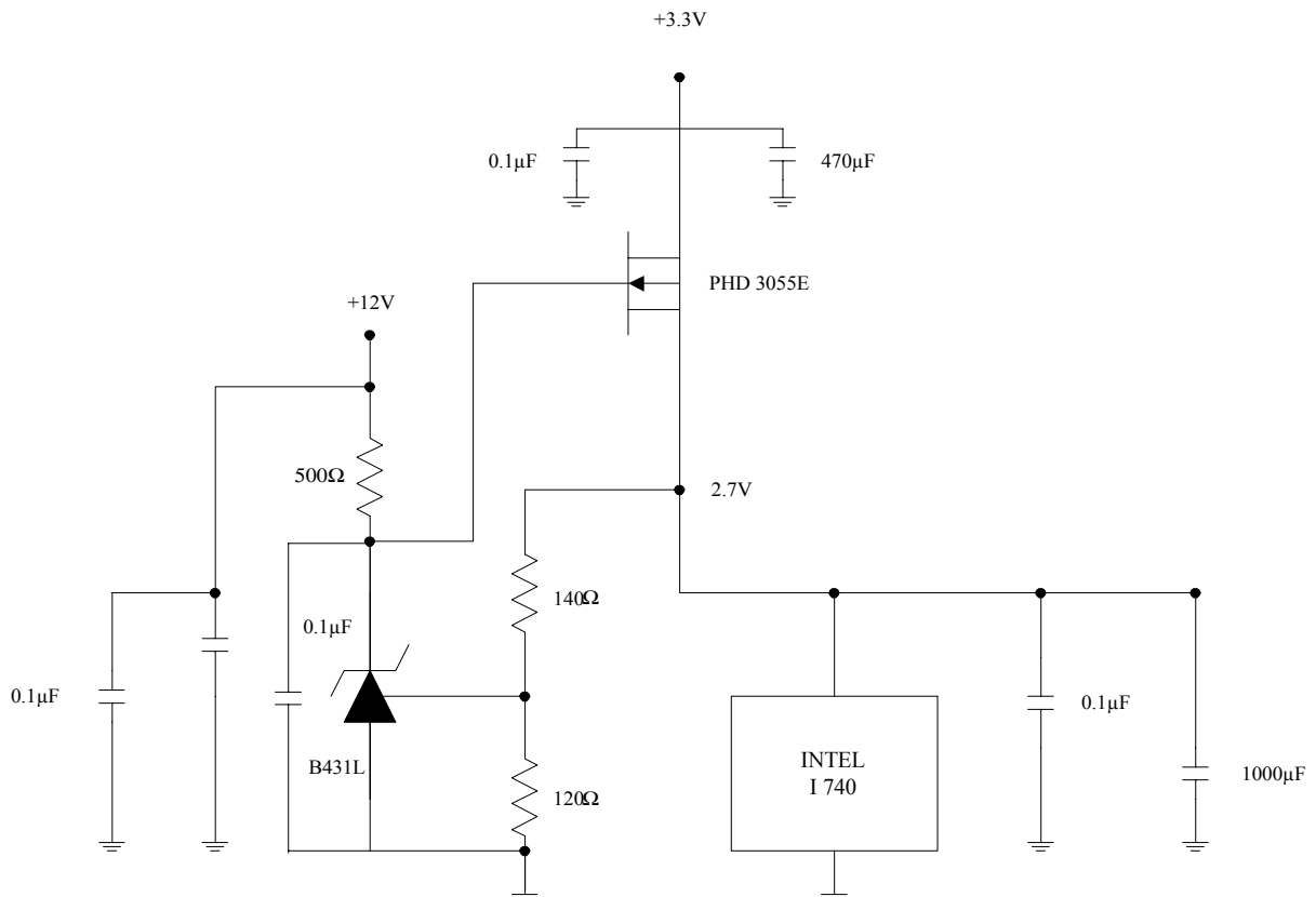
Test Circuit for I_{OFF}
