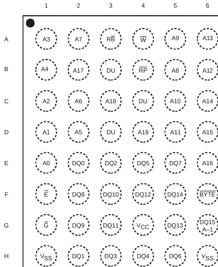
Figure 5. LFBGA Connections (Top view through package)
