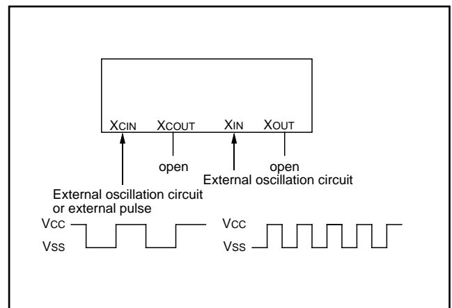
Fig. 80 External clock input circuit
