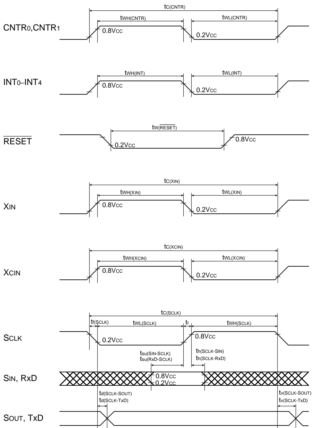
Fig. 103 Timing diagram
