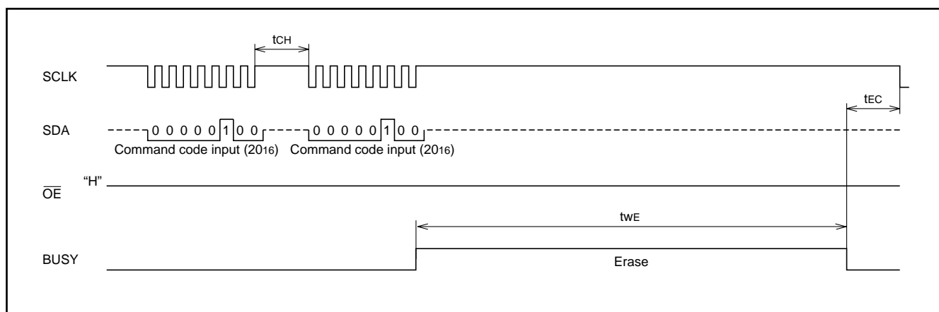
Fig. 95 Timings at erasing
