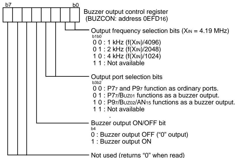
Fig. 75 Structure of buzzer output control register
