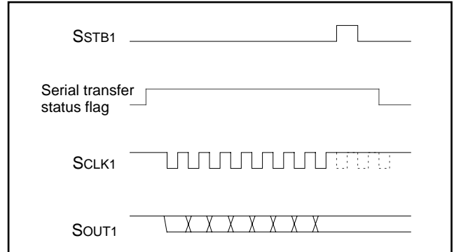
Fig. 26 S STB1 output operation
