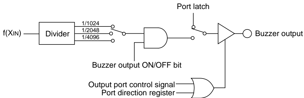
Fig. 74 Block diagram of buzzer output circuit
