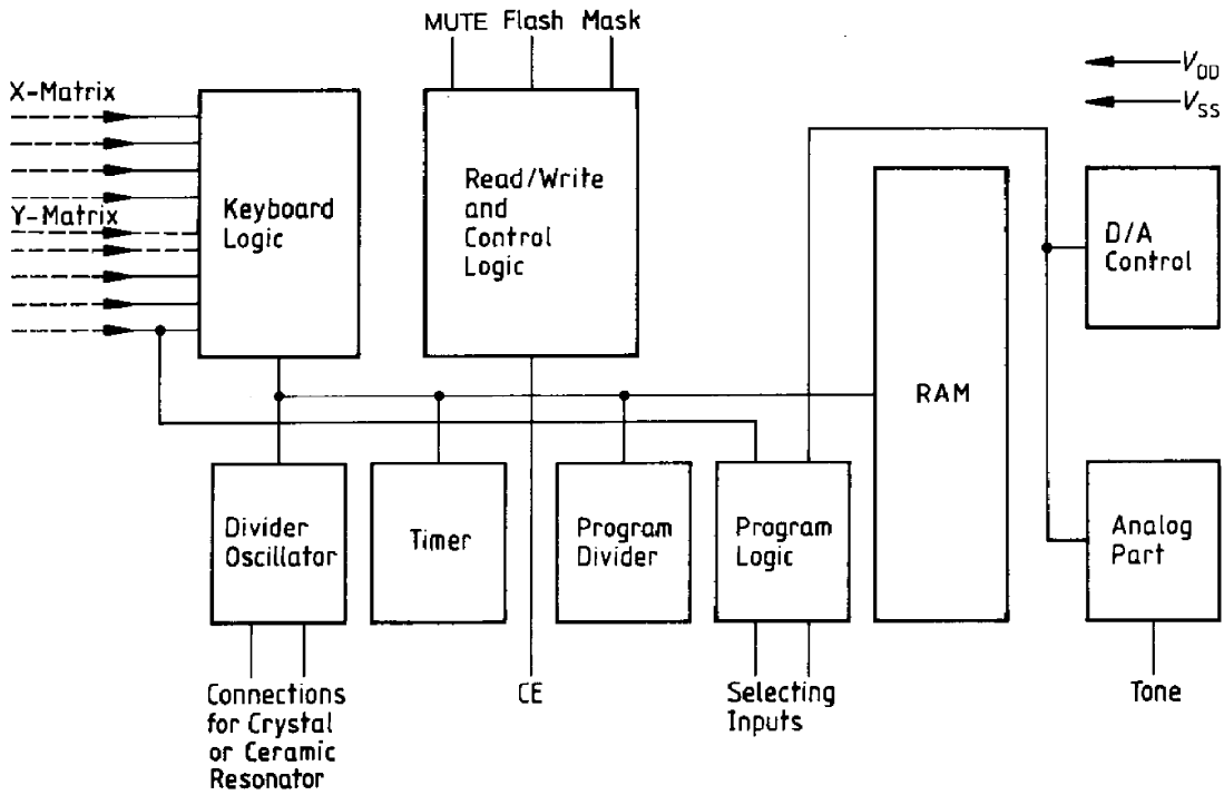
Block Diagram PSB 8510-X
