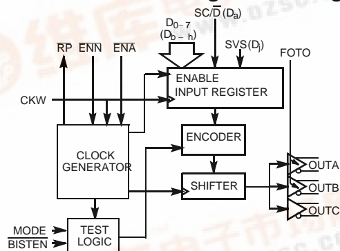
CY7B9234 Transmitter Logic Block Diagram
