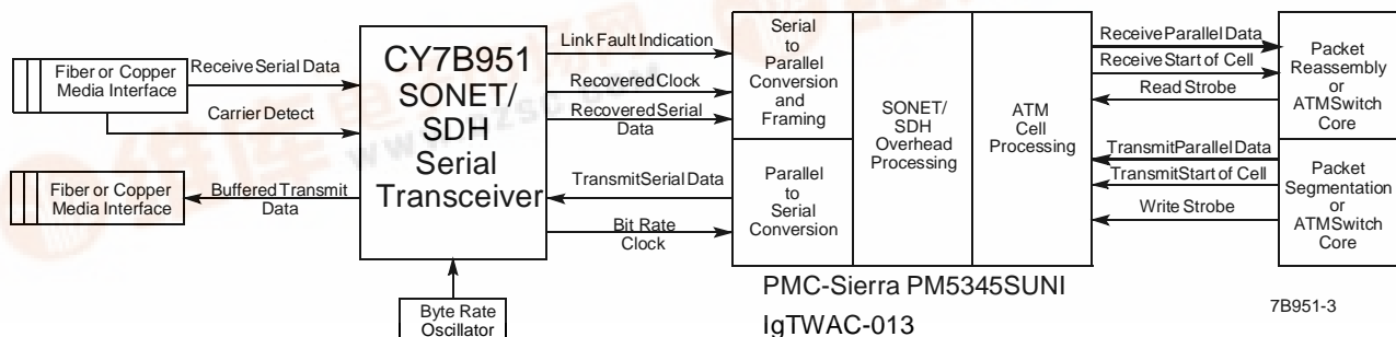
Figure 1. SONET/SDH and ATM Interface
