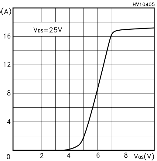
Transfer Characteristics
