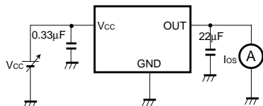
Fig. 5 Measurement circuit for output short-circuit current
