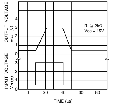
Fig.9 Output response characteristics
