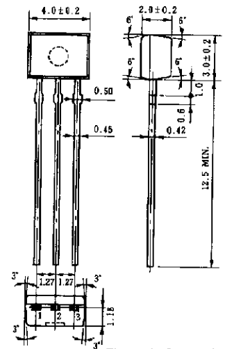
Electrode Connection
