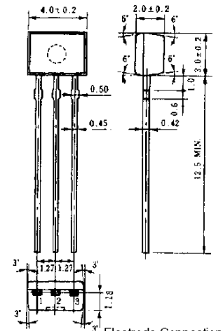
Electrode Connection 1. Emitter 2. Collector 3. Base
