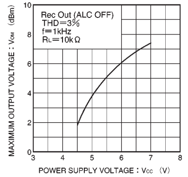
Fig. 8 Maximum output voltage vs. power supply voltage
