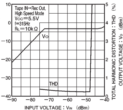
Fig. 13 Output voltage vs. input voltage
