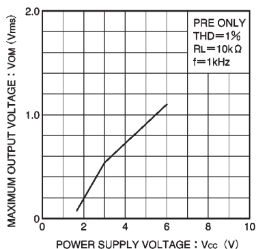
Fig. 22 Maximum output voltage vs. power supply voltage
