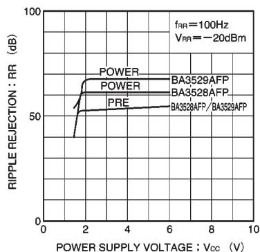
Fig. 21 Ripple rejection ratio vs. power supply voltage
