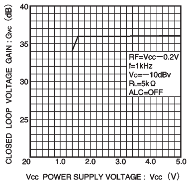
Fig. 13 Recording amp voltage gain vs. power supply voltage
