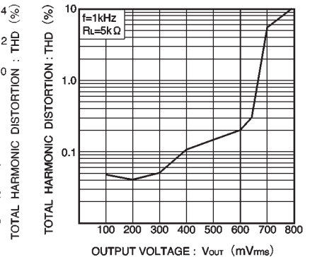
Fig. 8 Microphone amp total harmonic distortion vs. output voltage
