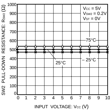
Fig. 11 SW2 pull-down resistance vs. power supply voltage
