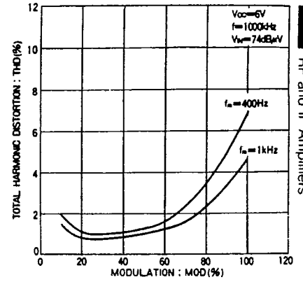
Fig. 33 AM total harmonic distortion vs. modulation frequency
