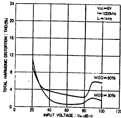
Fig. 29 AM total harmonic distortion vs. input voltage
