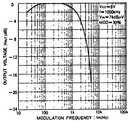
Fig. 34 AM detector output voltage vs. modulation frequency
