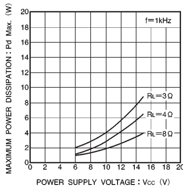
Fig. 16 Maximum power dissipation vs. power supply voltage
