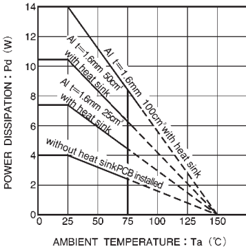
Fig. 3 Thermal derating curve
