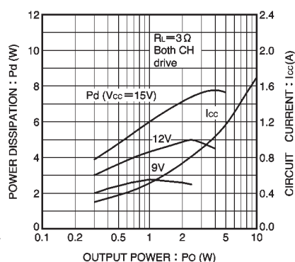
Fig. 30 Power dissipation and current vs. power supply voltage (RL = 3 Ohms)
