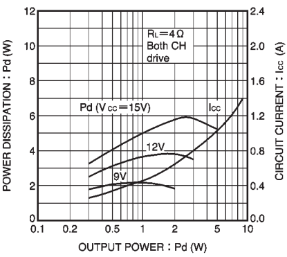
Fig. 31 Power dissipation and current dissipation vs. power supply voltage ( R_L = 4\Omega )
