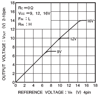
Fig.13 Output voltage vs. reference voltage ( II )
