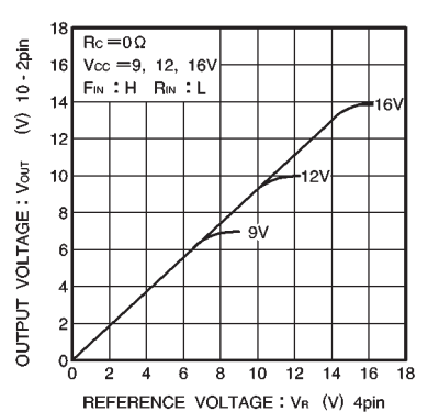
Fig.12 Output voltage vs. reference voltage ( I )
