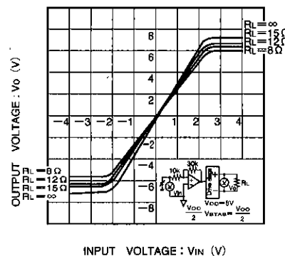
Fig. 7 Driver I/O characteristics (load variation)
