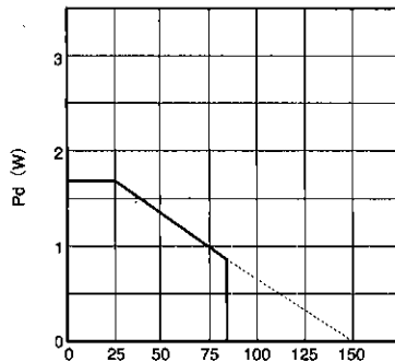
AMBIENT TEMPERATURE : Ta (°C) When mounted on 50 × 50 × 1.0 mm phenol paper PCB.
