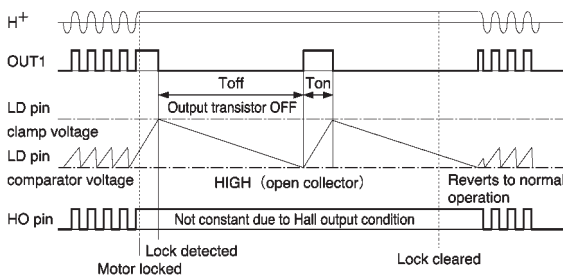
Fig.1 Timing chart of the LD and HO pins
