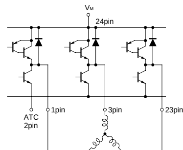
Fig.4 Output circuit
