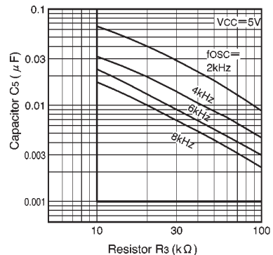
Range of the CR circuit connected to pin 9
