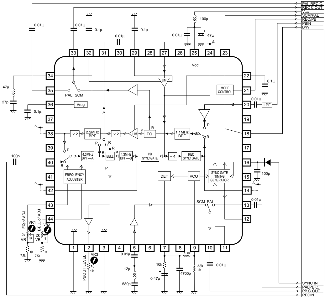
BA7207AK (QFP44)
