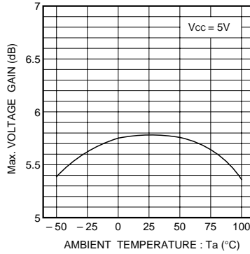
Fig. 4 Maximum voltage gain vs. ambient temperature
