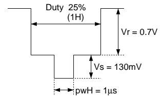
Duration of horizontal synchronization signal
