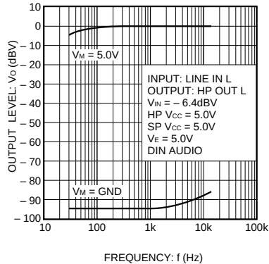
Fig. 7 HP AMP MUTE characteristics
