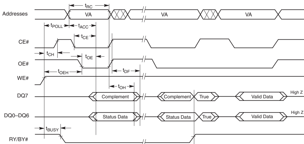
Figure I9. Data# Polling Timings (During Embedded Algorithms)
