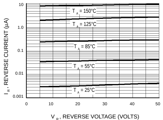
Figure 3. Leakage Current
