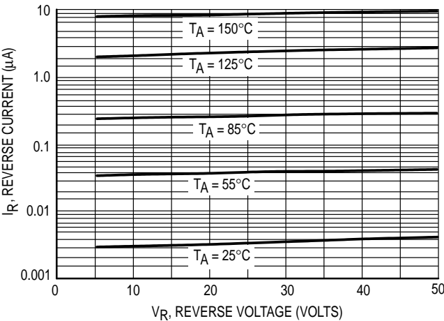
Figure 5. Leakage Current
