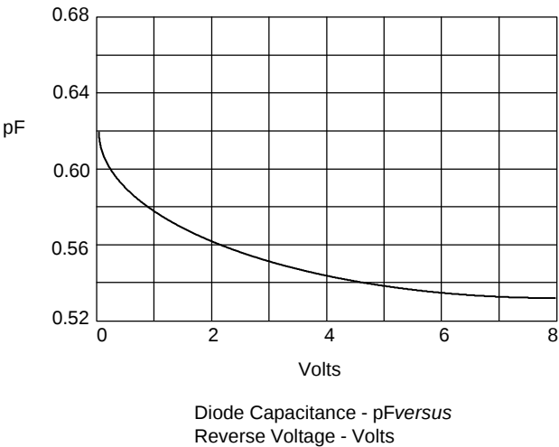
Figure 3 Diode Capacitance
