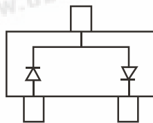
BAS40-04T Marking: 44
