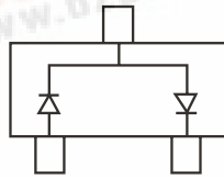
BAS40W-04 Marking: K44
