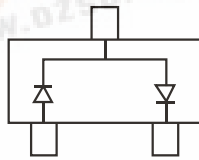
BAS70-04T Marking: 7D
