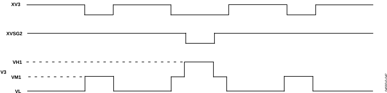
Figure 46. Example Showing V3 Output versus XV3 and XVSG2 Signals
