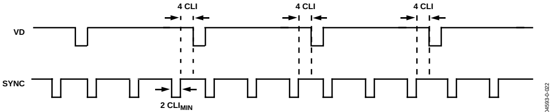
Figure 21. Example of Synchronization with SYNCPOL = 0 and SYNCCNT = 3
