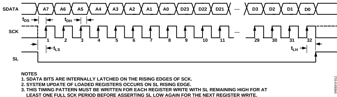
Figure 10. 3-Wire Serial Interface Timing for Control Registers
