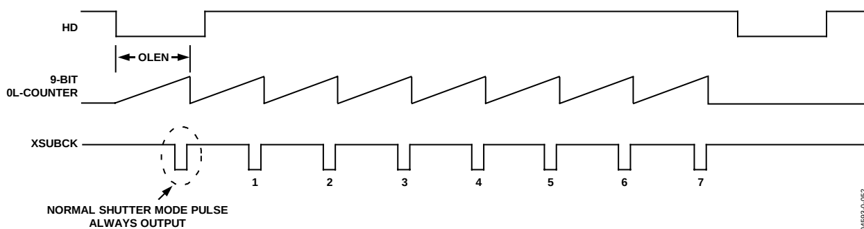
Figure 51. Electronic Shutter Timing
