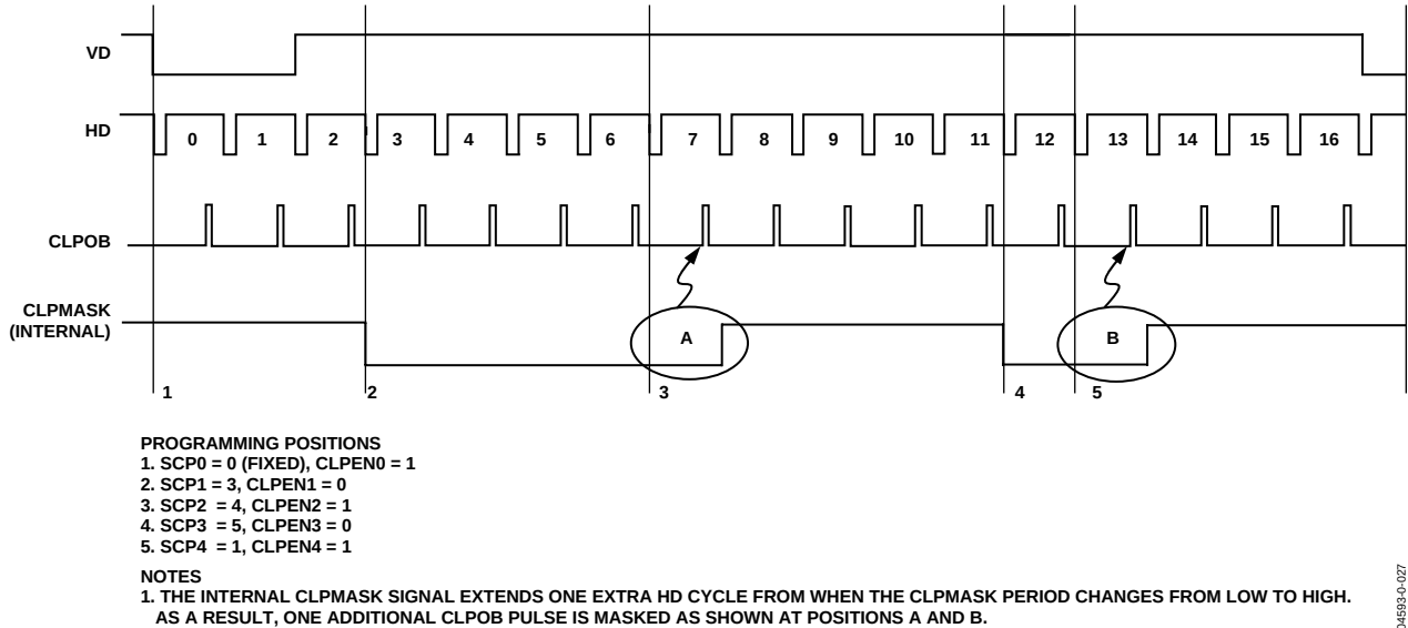
Figure 26. CLPOB Outputs with CLPMODE = 0
