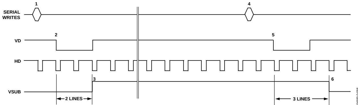
Figure 56. VSUB Timing Example
