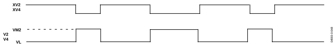
Figure 47. Example Showing V2 and V4 Outputs versus XV2 and XV4 Signals
