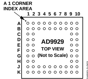
Figure 2. Pin Configuration
