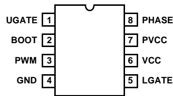
HIP6601BCB, HIP6603BCB (SOIC) HIP6601ECB, HIP6603ECB (EPSONIC) TOP VIEW
