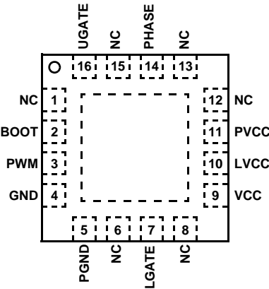
HIP6604B (QFN) TOP VIEW
