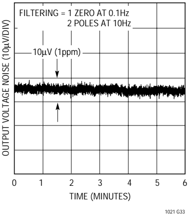
Output Noise 0.1Hz to 10Hz LT1021-10
