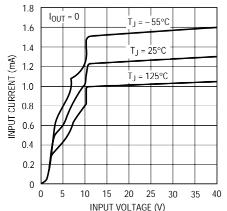
Input Supply Current LT1021-10
