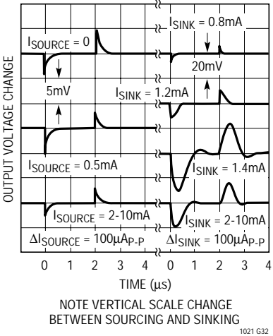
Load Transient Response LT1021-10, C_{LOAD} = 1000\text{pF}
