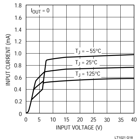
Quiescent Current LT1021-7
