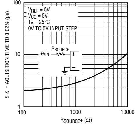
LTC1292/7 G15
