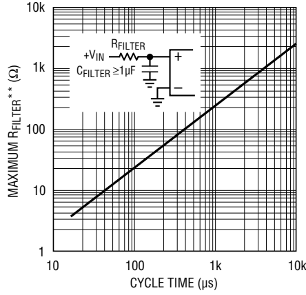
LTC1292/7 G14
