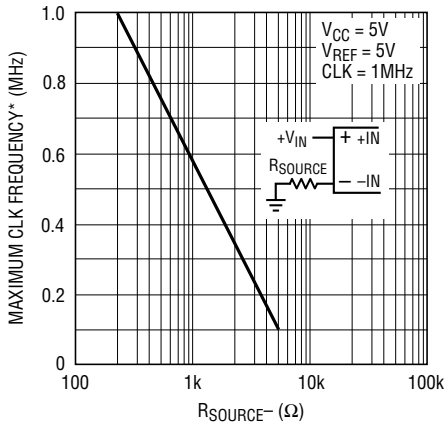
LTC1292/7 G13
