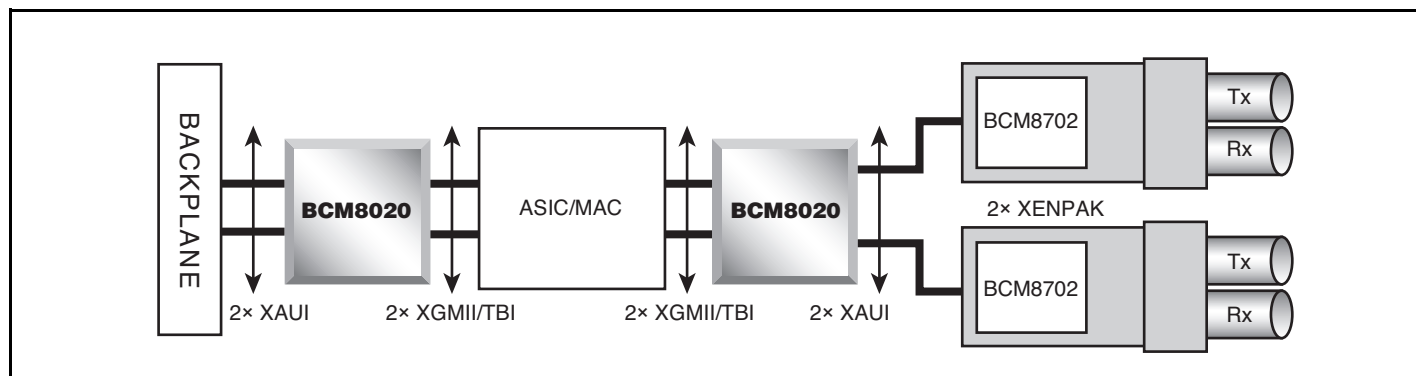
2 Independent Quad SerDes Application Diagram
