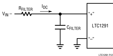
Figure 12. RC Input Filtering
