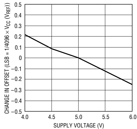
Change in Offset vs Supply Voltage
