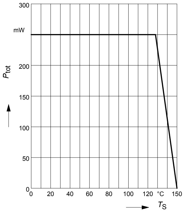
Total power dissipation P_{tot} = f(T_S) BCR164T
